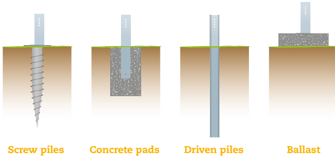
Screw piles
